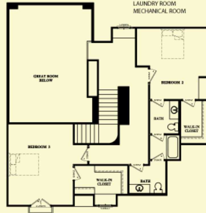
A7 SECOND FLOOR
