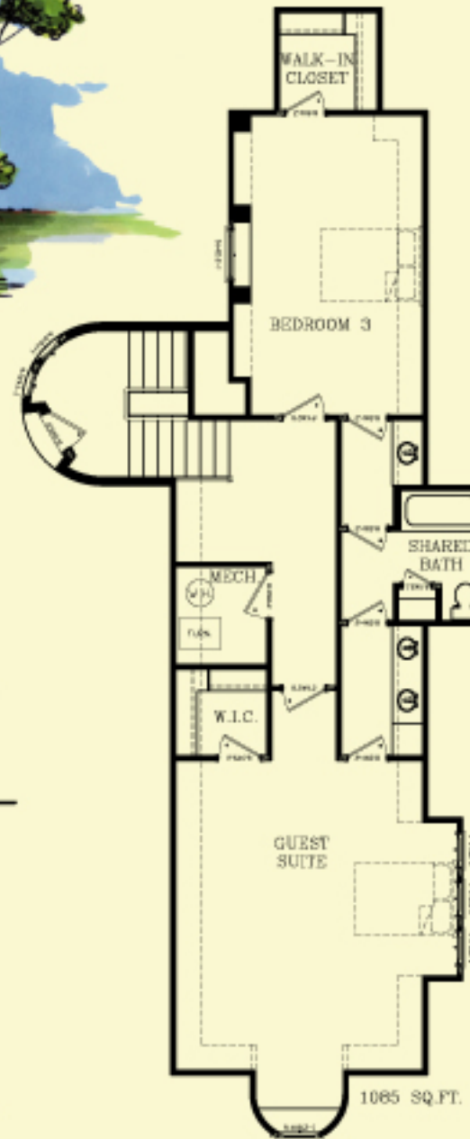
A7 SECOND FLOOR
