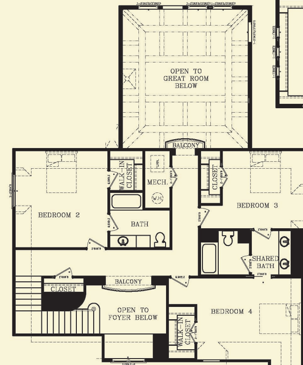
A7 SECOND FLOOR
